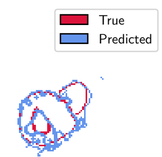
segmentations
